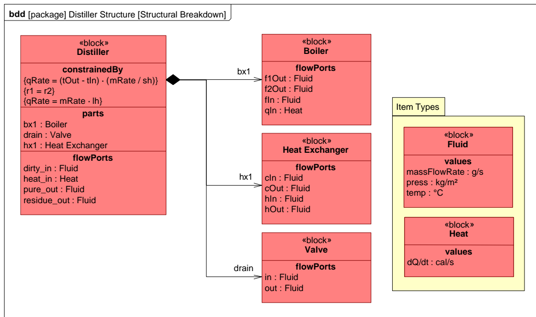
Figure 7: Block Definition Diagram
