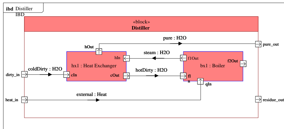
Figure 8: IBD for Distiller
