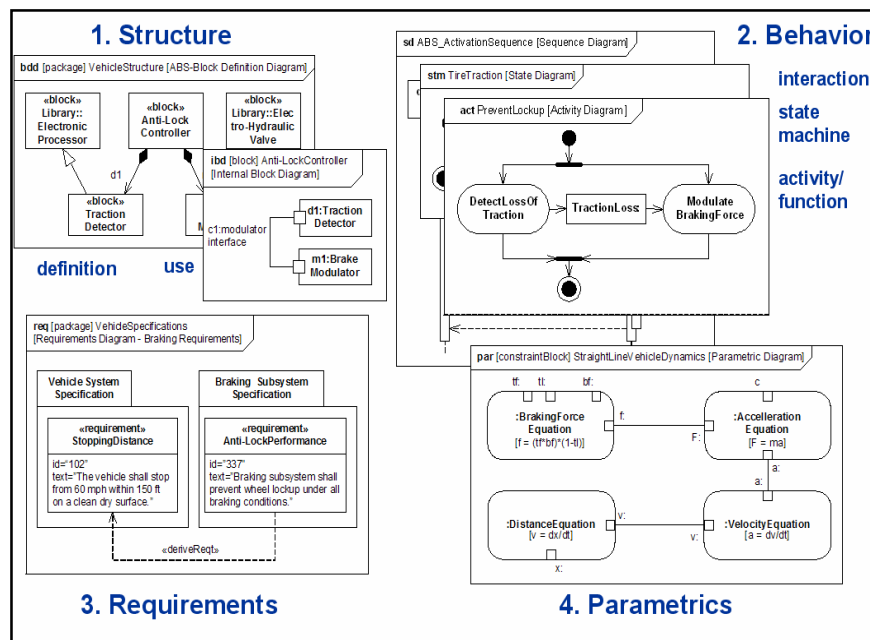
Figure 4: The Four Pillars of OMG SysML
