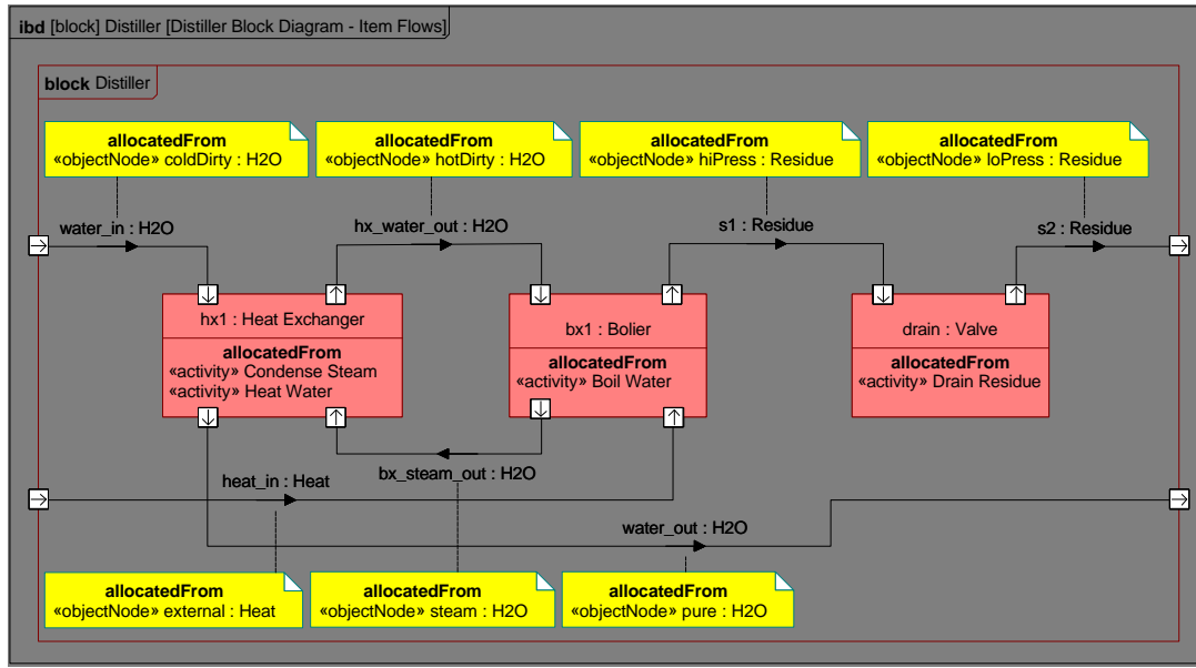
Figure 11: Structure Diagram Allocation
