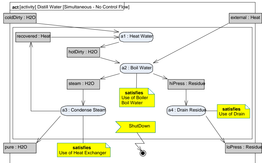
Figure 6: Distill Water Activity with Requirements
