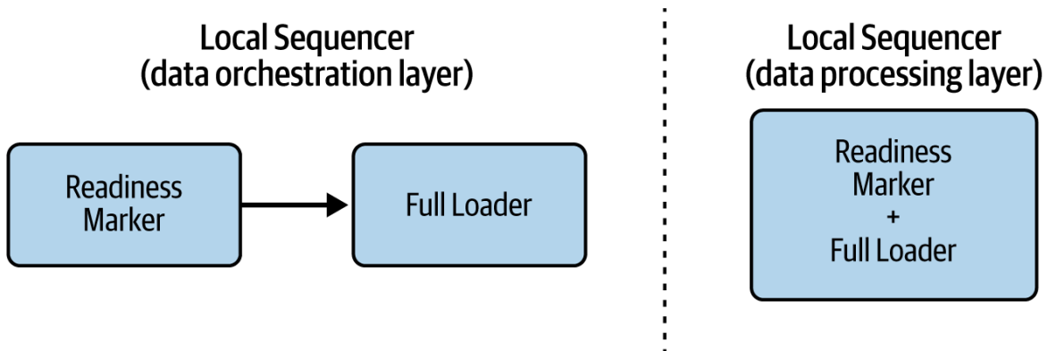
Figure 6-1. Local Sequencer versus single task
