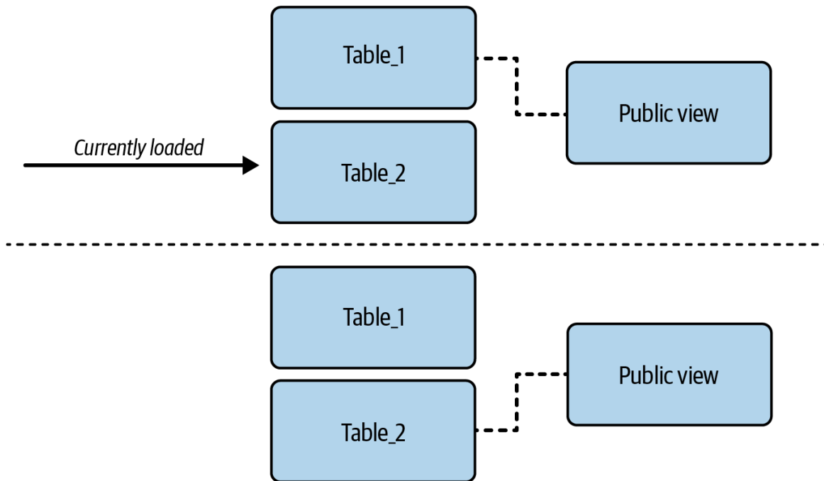
Figure 2-1. Single data exposition abstraction example with a database view
