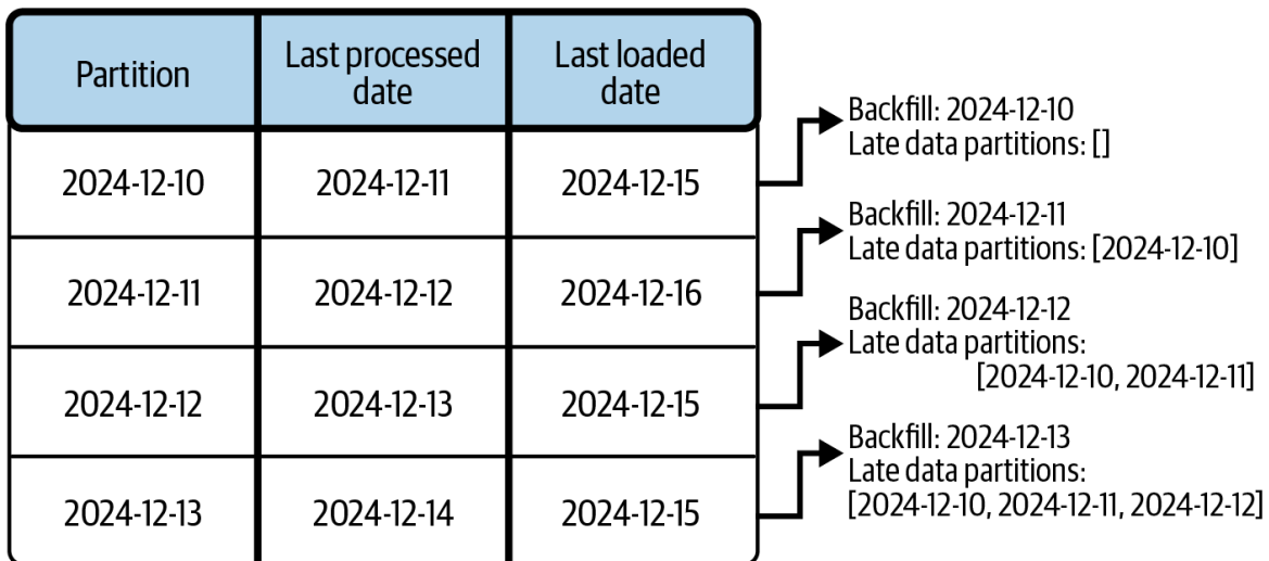
Figure 3-9. Late data integration concurrency problem
