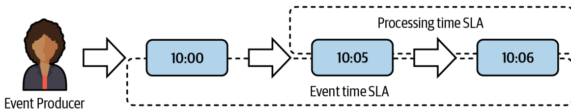
Figure 10-2. Processing time and event time SLAs illustrated
