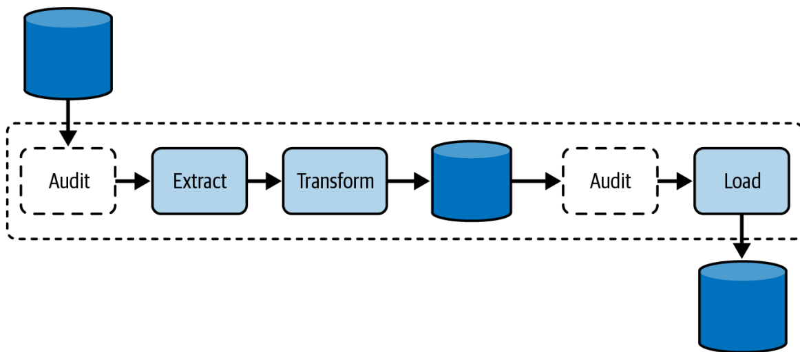
Figure 9-1. The AWAP pattern applied to a pipeline
