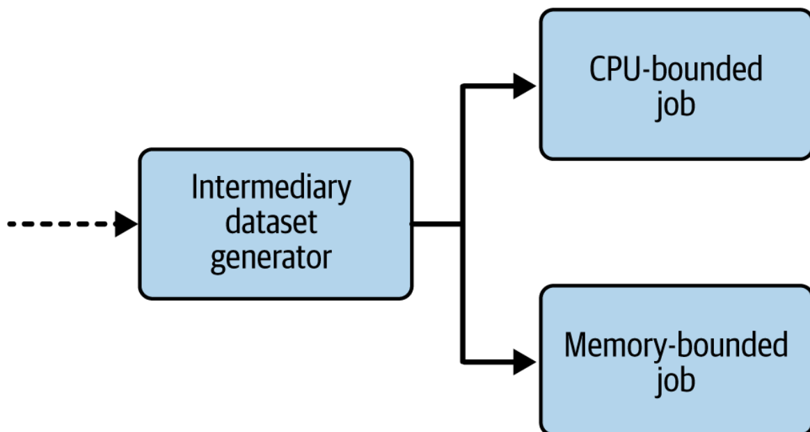
Figure 6-5. Splitting a job working on the same base dataset but requiring different compute capacity (dashed arrow indicates previous tasks in the pipeline not relevant to this example)
