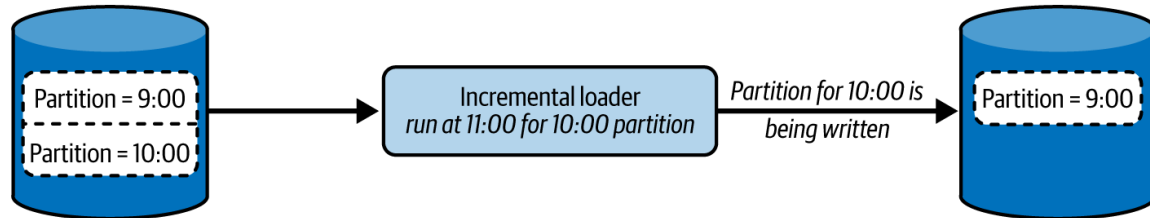
Figure 2-2. Two possible implementations of the Incremental Loader pattern
