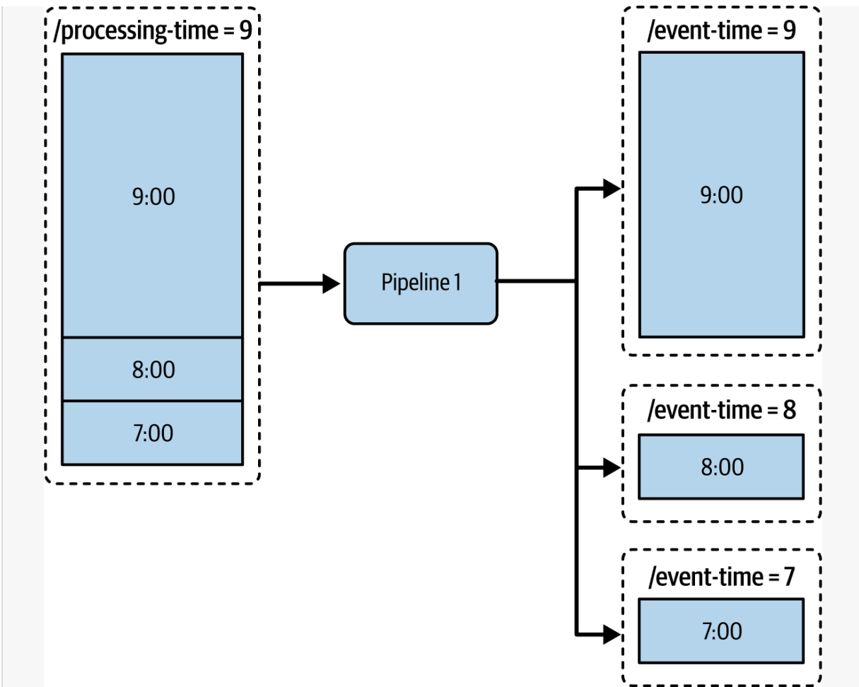
Figure 3-5. Shifting the late data problem
