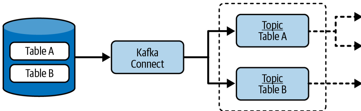
Figure 2-3. Debezium architecture in a nutshell, showing a Kafka Connect consumer leveraging the database commit logs and writing all matching datasets to dedicated Apache Kafka topics
